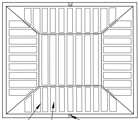
ALL BARS 5/8" ALL SLOTS 1" PLAN VIEW N.T.S. SLOT FOR LOCKING BOLT
