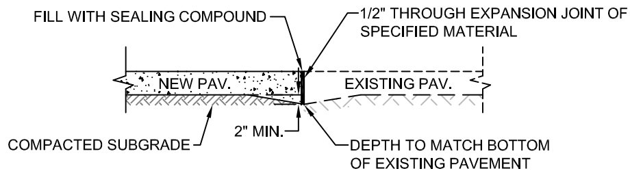
EXPANSION JOINT BETWEEN OLD AND NEW CONSTRUCTION
