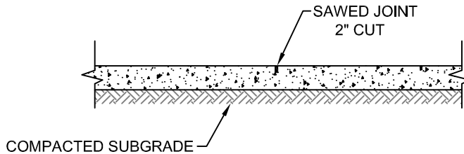
CONSTRUCTION CONTROL JOINT LONGITUDINAL OR TRANSVERSE
