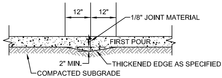
CONSTRUCTION JOINT LONGITUDINAL OR TRANSVERSE
